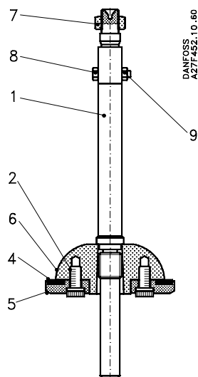
Fig. 1, Push rod assembly for PM 3, sizes 80 to 125
