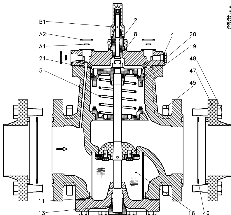
Fig. 2, PM 3, sizes 80 to 125
